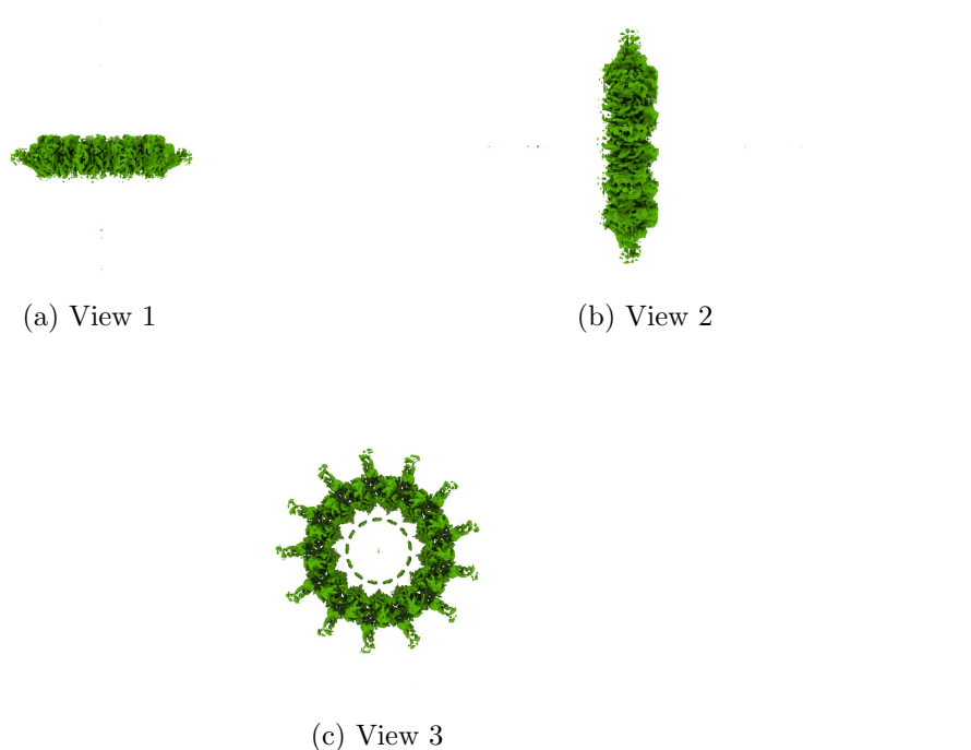
Figure 4: Isosurface at threshold=0.080000. Views generated by ChimeraX at a the following X, Y, Z angles: View 1 (0, -90, -90), View 2 (-90, 0, -90), View 3 (0, 0, 0).
