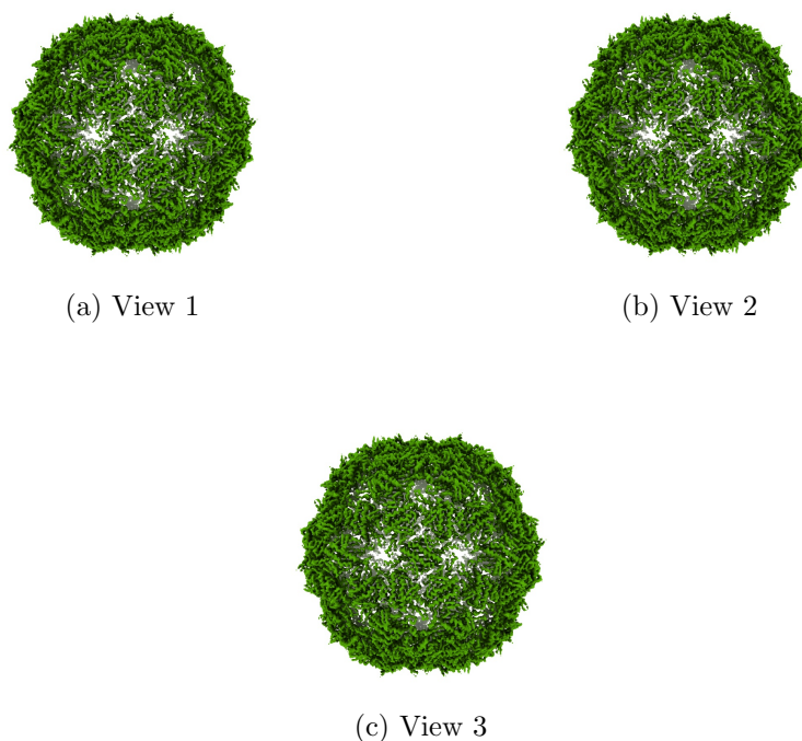
Figure 4: Isosurface at threshold=0.528000. Views generated by ChimeraX at the following X, Y, Z angles: View 1 (0, -90, -90), View 2 (-90, 0, -90), View 3 (0, 0, 0).
