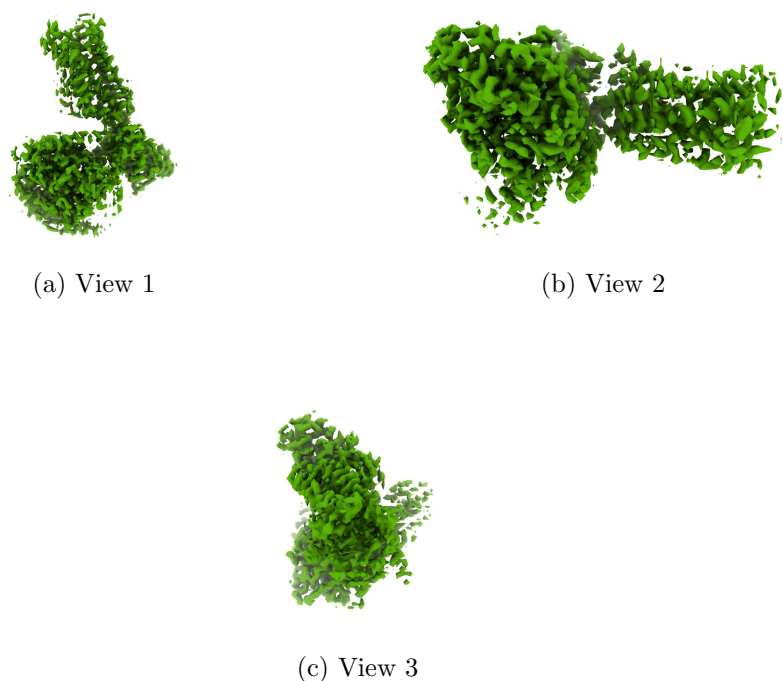
Figure 4: Isosurface at threshold=0.374000. Views generated by ChimeraX at a the following X, Y, Z angles: View 1 (0, -90, -90), View 2 (-90, 0, -90), View 3 (0, 0, 0).
