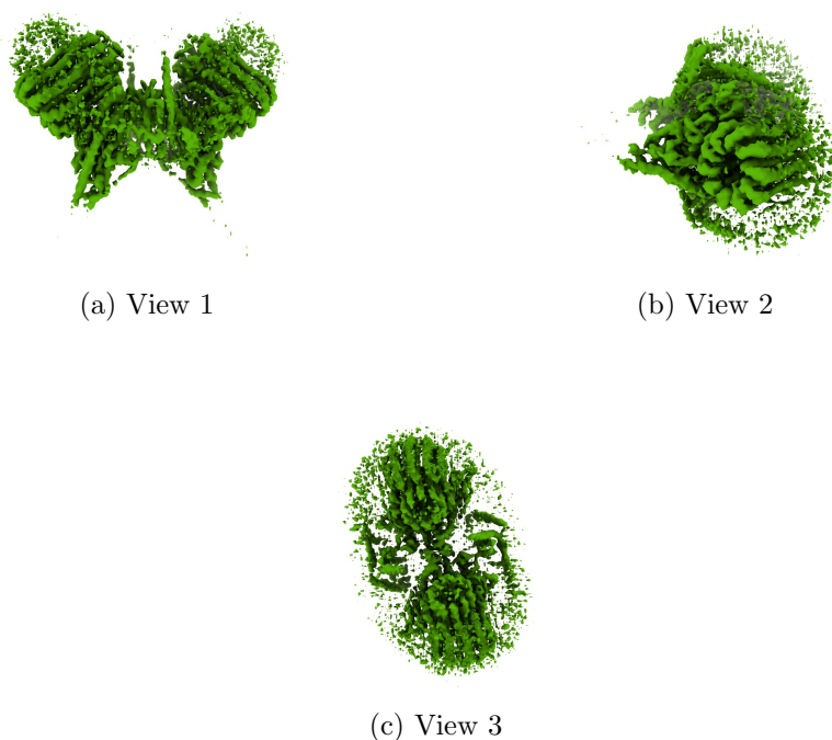
Figure 4: Isosurface at threshold=0.162000. Views generated by ChimeraX at a the following X, Y, Z angles: View 1 (0, -90, -90), View 2 (-90, 0, -90), View 3 (0, 0, 0).
