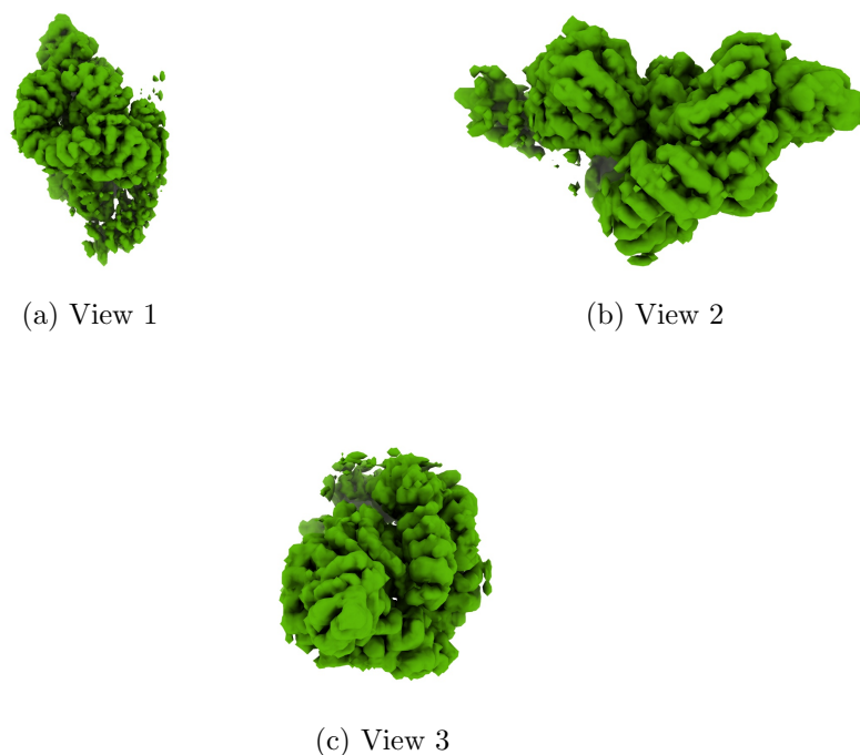
Figure 4: Isosurface at threshold=0.052600. Views generated by ChimeraX at a the following X, Y, Z angles: View 1 (0, -90, -90), View 2 (-90, 0, -90), View 3 (0, 0, 0).
