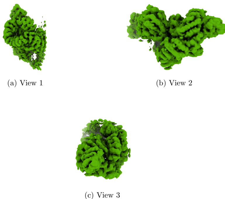
Figure 4: Isosurface at threshold=0.051300. Views generated by ChimeraX at a the following X, Y, Z angles: View 1 (0, -90, -90), View 2 (-90, 0, -90), View 3 (0, 0, 0).
