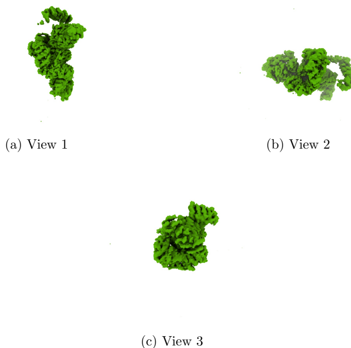
Figure 4: Isosurface at threshold=0.016700. Views generated by ChimeraX at a the following X, Y, Z angles: View 1 (0, -90, -90), View 2 (-90, 0, -90), View 3 (0, 0, 0).
