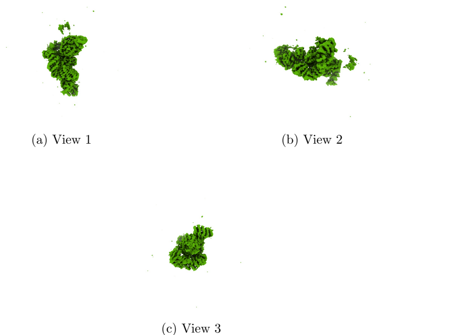
Figure 4: Isosurface at threshold=0.139000. Views generated by ChimeraX at a the following X, Y, Z angles: View 1 (0, -90, -90), View 2 (-90, 0, -90), View 3 (0, 0, 0).
