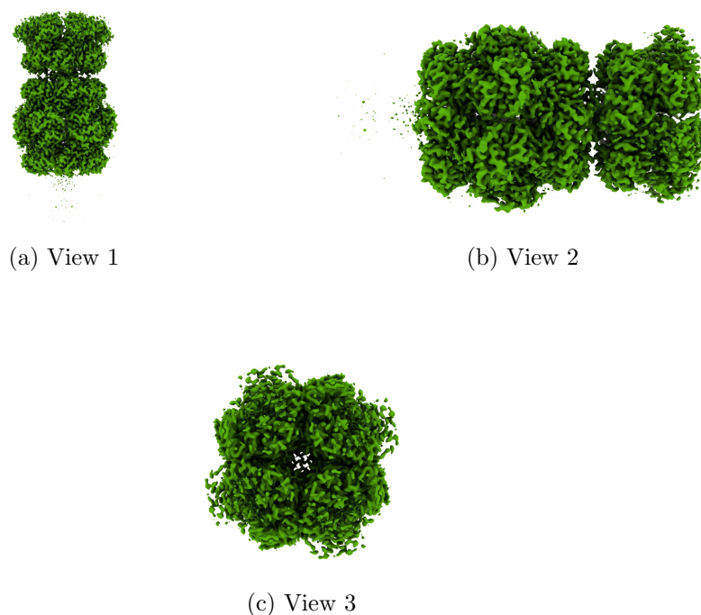
Figure 4: Isosurface at threshold=0.255000. Views generated by ChimeraX at a the following X, Y, Z angles: View 1 (0, -90, -90), View 2 (-90, 0, -90), View 3 (0, 0, 0).
