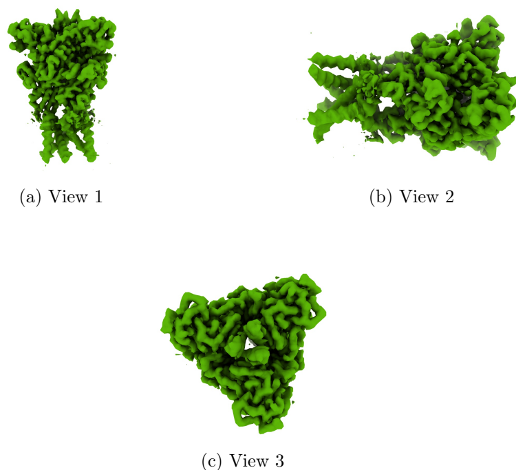
Figure 4: Isosurface at threshold=0.042800. Views generated by ChimeraX at a the following X, Y, Z angles: View 1 (0, -90, -90), View 2 (-90, 0, -90), View 3 (0, 0, 0).
