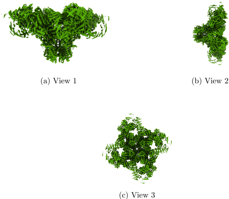
Figure 4: Isosurface at threshold=0.047000. Views generated by ChimeraX at a the following X, Y, Z angles: View 1 (0, -90, -90), View 2 (-90, 0, -90), View 3 (0, 0, 0).
