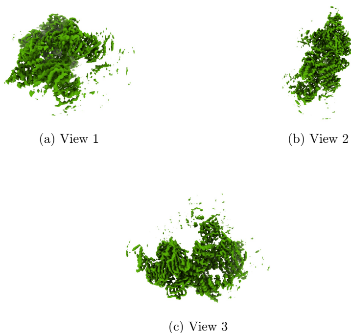
Figure 4: Isosurface at threshold=0.061000. Views generated by ChimeraX at a the following X, Y, Z angles: View 1 (0, -90, -90), View 2 (-90, 0, -90), View 3 (0, 0, 0).
