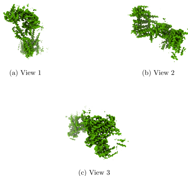
Figure 4: Isosurface at threshold=0.167000. Views generated by ChimeraX at a the following X, Y, Z angles: View 1 (0, -90, -90), View 2 (-90, 0, -90), View 3 (0, 0, 0).
