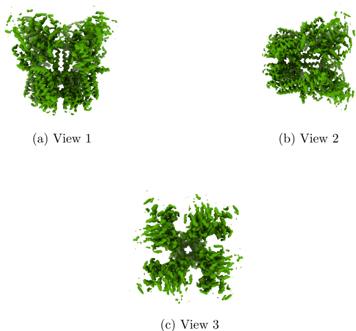
Figure 4: Isosurface at threshold=0.154000. Views generated by ChimeraX at a the following X, Y, Z angles: View 1 (0, -90, -90), View 2 (-90, 0, -90), View 3 (0, 0, 0).
