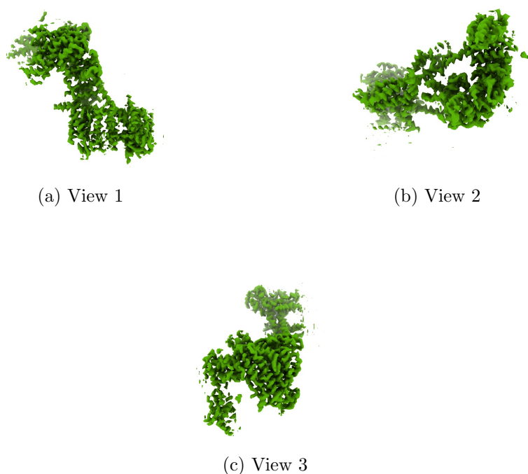
Figure 4: Isosurface at threshold=0.174000. Views generated by ChimeraX at a the following X, Y, Z angles: View 1 (0, -90, -90), View 2 (-90, 0, -90), View 3 (0, 0, 0).
