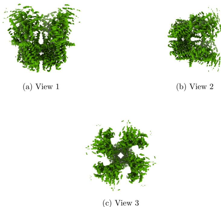
Figure 4: Isosurface at threshold=0.157000. Views generated by ChimeraX at a the following X, Y, Z angles: View 1 (0, -90, -90), View 2 (-90, 0, -90), View 3 (0, 0, 0).
