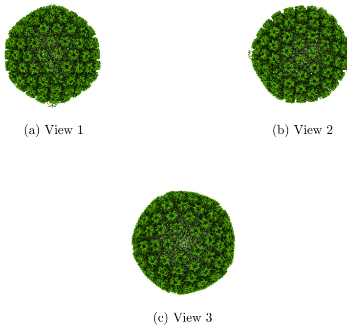
Figure 4: Isosurface at threshold=0.870000. Views generated by ChimeraX at a the following X, Y, Z angles: View 1 (0, -90, -90), View 2 (-90, 0, -90), View 3 (0, 0, 0).
