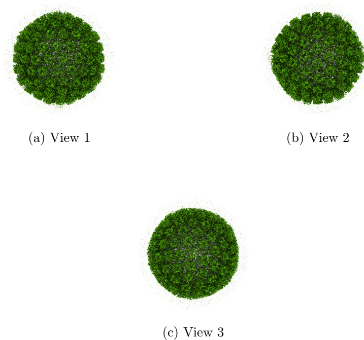
Figure 4: Isosurface at threshold=1.910000. Views generated by ChimeraX at a the following X, Y, Z angles: View 1 (0, -90, -90), View 2 (-90, 0, -90), View 3 (0, 0, 0).
