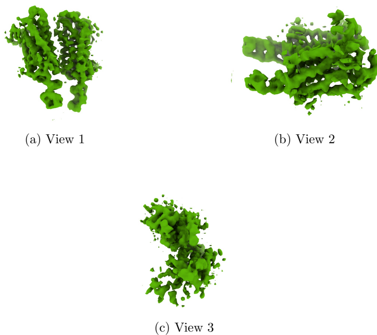
Figure 4: Isosurface at threshold=0.875000. Views generated by ChimeraX at a the following X, Y, Z angles: View 1 (0, -90, -90), View 2 (-90, 0, -90), View 3 (0, 0, 0).
