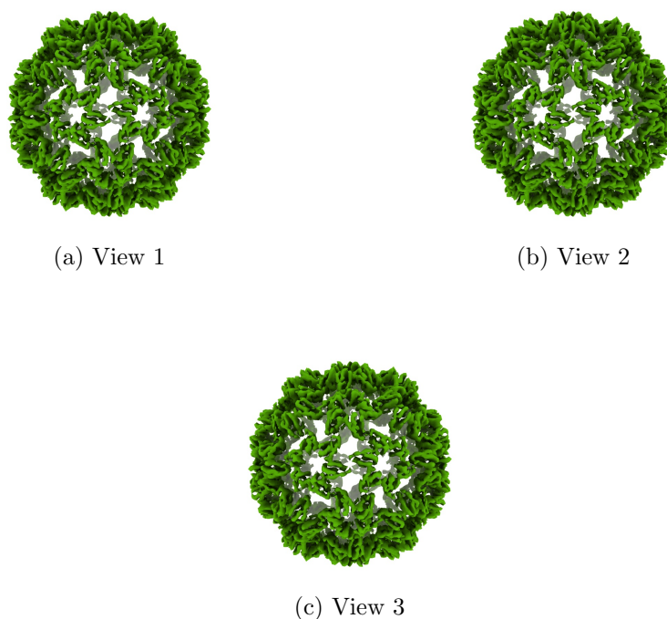
Figure 4: Isosurface at threshold=0.067400. Views generated by ChimeraX at a the following X, Y, Z angles: View 1 (0, -90, -90), View 2 (-90, 0, -90), View 3 (0, 0, 0).
