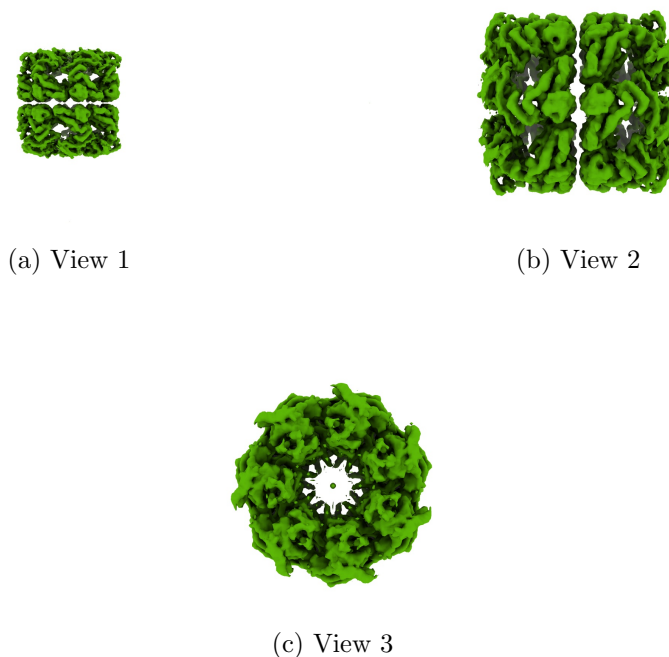
Figure 4: Isosurface at threshold=0.063600. Views generated by ChimeraX at a the following X, Y, Z angles: View 1 (0, -90, -90), View 2 (-90, 0, -90), View 3 (0, 0, 0).
