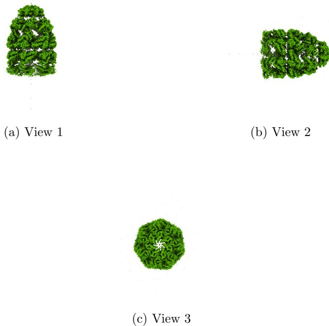
Figure 4: Isosurface at threshold=0.086400. Views generated by ChimeraX at a the following X, Y, Z angles: View 1 (0, -90, -90), View 2 (-90, 0, -90), View 3 (0, 0, 0).
