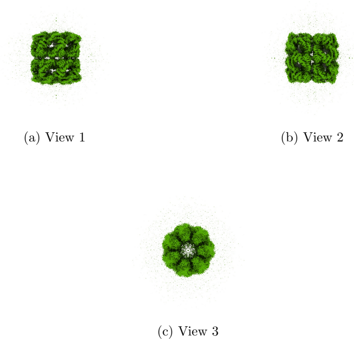
Figure 4: Isosurface at threshold=0.056600. Views generated by ChimeraX at a the following X, Y, Z angles: View 1 (0, -90, -90), View 2 (-90, 0, -90), View 3 (0, 0, 0).
