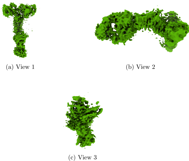
Figure 4: Isosurface at threshold=0.596000. Views generated by ChimeraX at a the following X, Y, Z angles: View 1 (0, -90, -90), View 2 (-90, 0, -90), View 3 (0, 0, 0).
