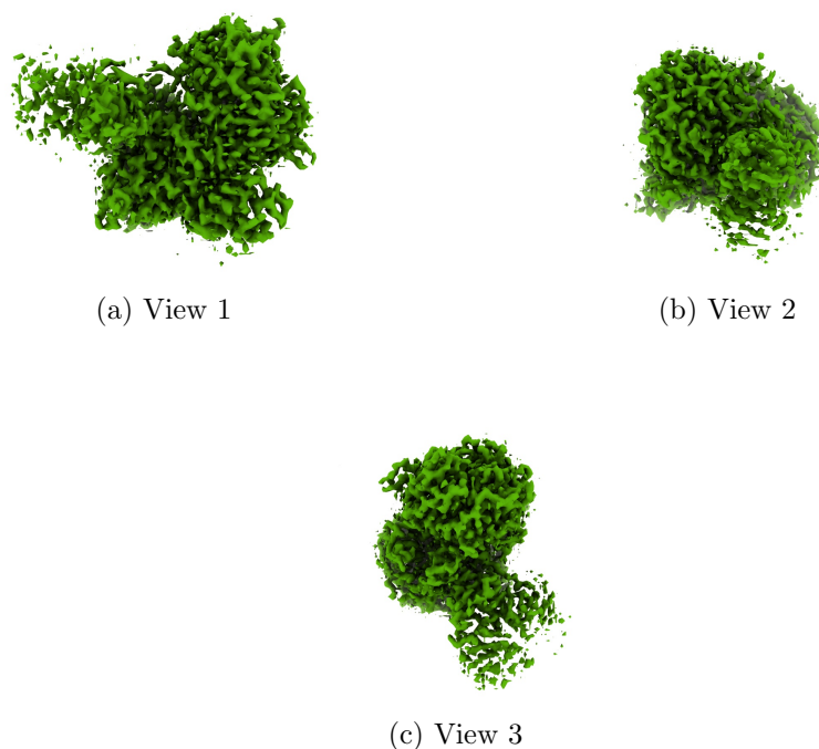
Figure 4: Isosurface at threshold=0.144000. Views generated by ChimeraX at a the following X, Y, Z angles: View 1 (0, -90, -90), View 2 (-90, 0, -90), View 3 (0, 0, 0).
