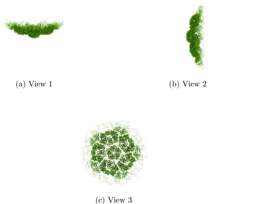
Figure 4: Isosurface at threshold=0.030000. Views generated by ChimeraX at a the following X, Y, Z angles: View 1 (0, -90, -90), View 2 (-90, 0, -90), View 3 (0, 0, 0).
