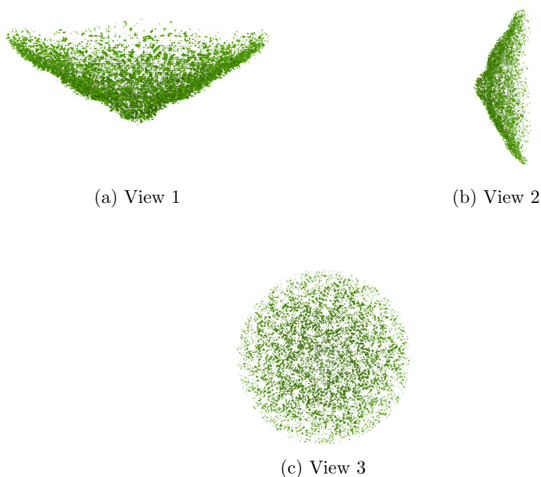
Figure 4: Isosurface at threshold=0.005000. Views generated by ChimeraX at a the following X, Y, Z angles: View 1 (0, -90, -90), View 2 (-90, 0, -90), View 3 (0, 0, 0).
