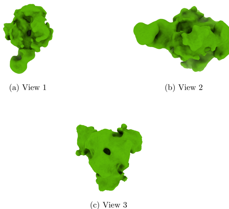
Figure 4: Isosurface at threshold=0.007480. Views generated by ChimeraX at a the following X, Y, Z angles: View 1 (0, -90, -90), View 2 (-90, 0, -90), View 3 (0, 0, 0).
