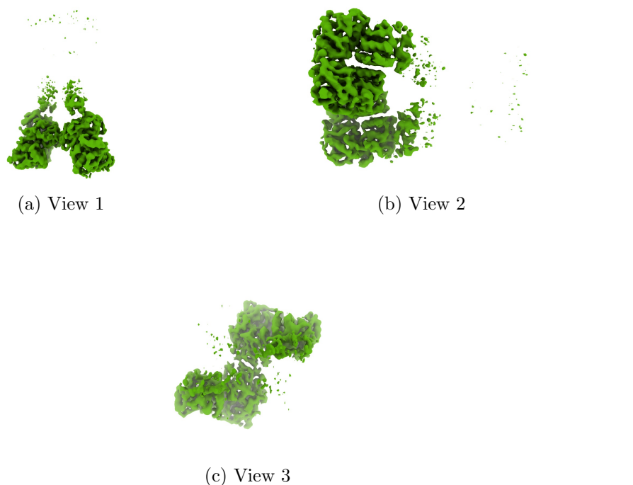
Figure 4: Isosurface at threshold=0.300000. Views generated by ChimeraX at a the following X, Y, Z angles: View 1 (0, -90, -90), View 2 (-90, 0, -90), View 3 (0, 0, 0).
