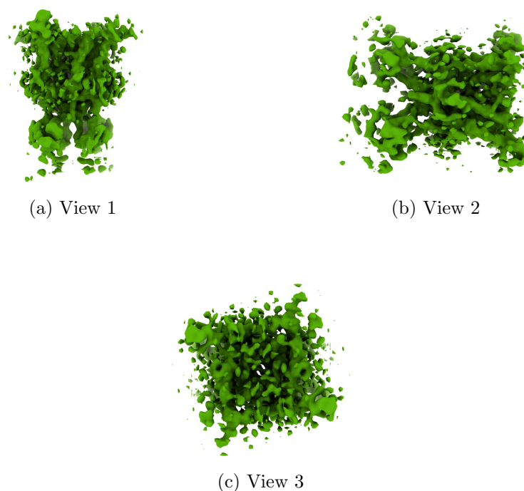
Figure 4: Isosurface at threshold=0.300000. Views generated by ChimeraX at the following X, Y, Z angles: View 1 (0, -90, -90), View 2 (-90, 0, -90), View 3 (0, 0, 0).
