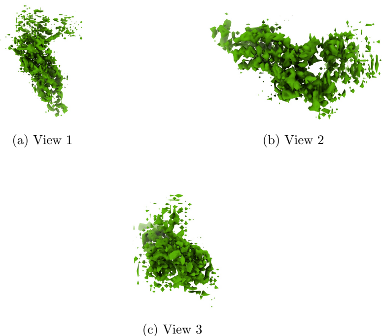
Figure 4: Isosurface at threshold=0.512000. Views generated by ChimeraX at a the following X, Y, Z angles: View 1 (0, -90, -90), View 2 (-90, 0, -90), View 3 (0, 0, 0).
