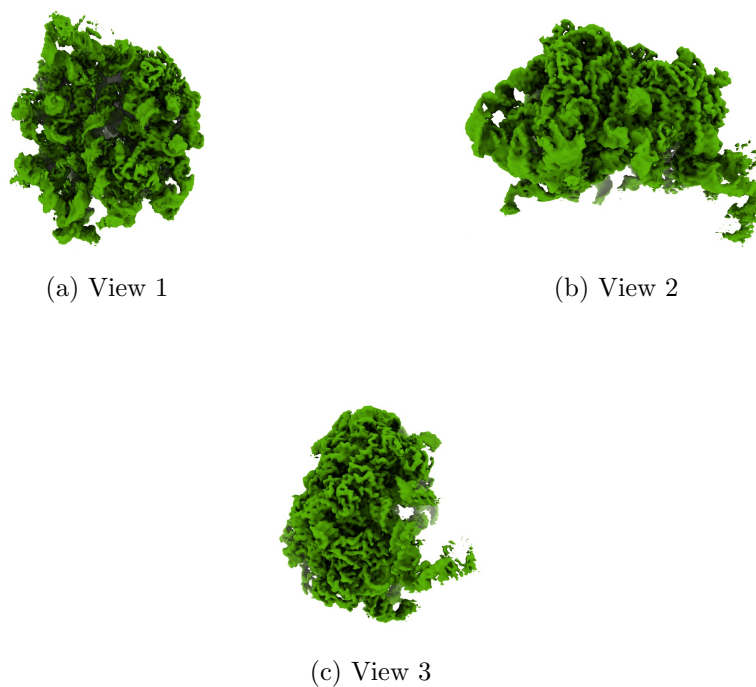
Figure 4: Isosurface at threshold=0.436000. Views generated by ChimeraX at a the following X, Y, Z angles: View 1 (0, -90, -90), View 2 (-90, 0, -90), View 3 (0, 0, 0).
