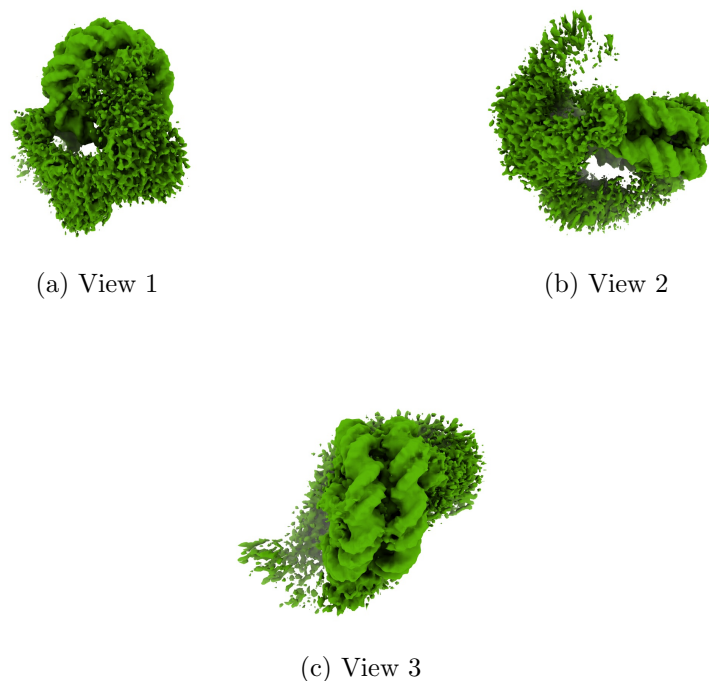
Figure 4: Isosurface at threshold=0.107000. Views generated by ChimeraX at a the following X, Y, Z angles: View 1 (0, -90, -90), View 2 (-90, 0, -90), View 3 (0, 0, 0).
