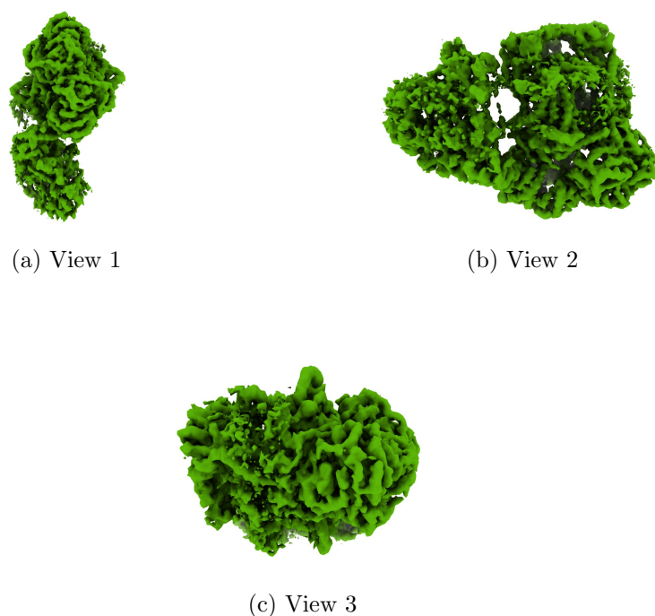
Figure 4: Isosurface at threshold=0.115000. Views generated by ChimeraX at a the following X, Y, Z angles: View 1 (0, -90, -90), View 2 (-90, 0, -90), View 3 (0, 0, 0).
