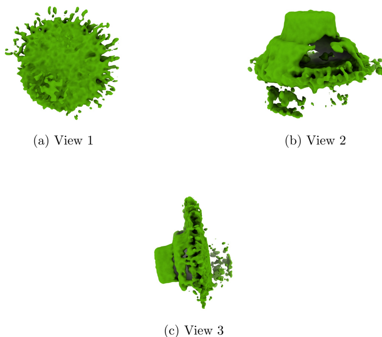
Figure 4: Isosurface at threshold=0.095700. Views generated by ChimeraX at a the following X, Y, Z angles: View 1 (0, -90, -90), View 2 (-90, 0, -90), View 3 (0, 0, 0).
