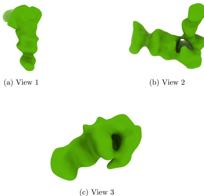
Figure 4: Isosurface at threshold=0.865000. Views generated by ChimeraX at a the following X, Y, Z angles: View 1 (0, -90, -90), View 2 (-90, 0, -90), View 3 (0, 0, 0).
