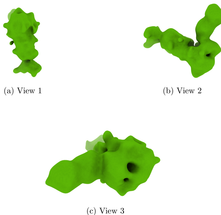
Figure 4: Isosurface at threshold=0.940000. Views generated by ChimeraX at a the following X, Y, Z angles: View 1 (0, -90, -90), View 2 (-90, 0, -90), View 3 (0, 0, 0).
