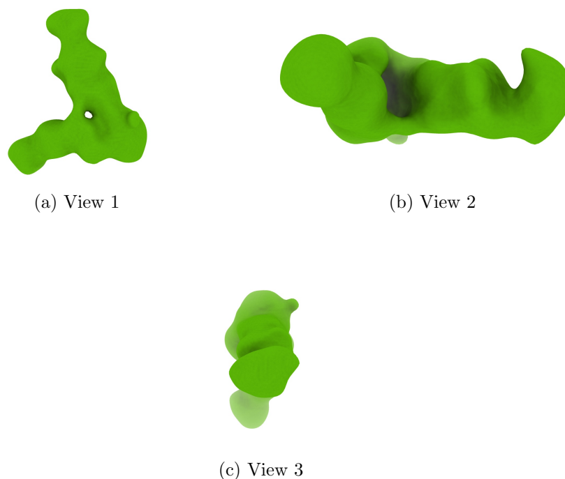
Figure 4: Isosurface at threshold=0.880000. Views generated by ChimeraX at a the following X, Y, Z angles: View 1 (0, -90, -90), View 2 (-90, 0, -90), View 3 (0, 0, 0).
