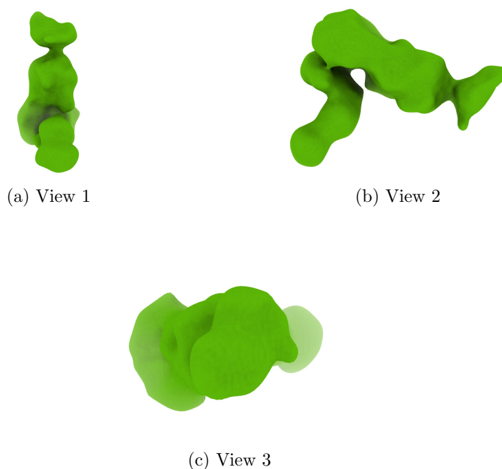
Figure 4: Isosurface at threshold=1.150000. Views generated by ChimeraX at a the following X, Y, Z angles: View 1 (0, -90, -90), View 2 (-90, 0, -90), View 3 (0, 0, 0).
