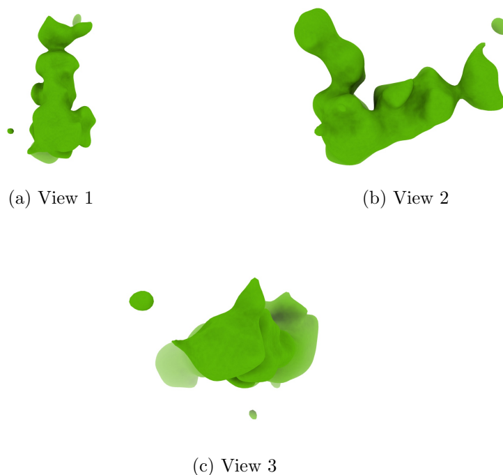
Figure 4: Isosurface at threshold=1.340000. Views generated by ChimeraX at a the following X, Y, Z angles: View 1 (0, -90, -90), View 2 (-90, 0, -90), View 3 (0, 0, 0).
