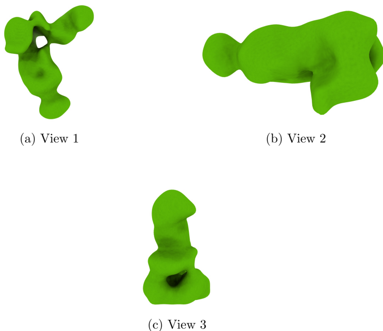
Figure 4: Isosurface at threshold=0.908000. Views generated by ChimeraX at a the following X, Y, Z angles: View 1 (0, -90, -90), View 2 (-90, 0, -90), View 3 (0, 0, 0).
