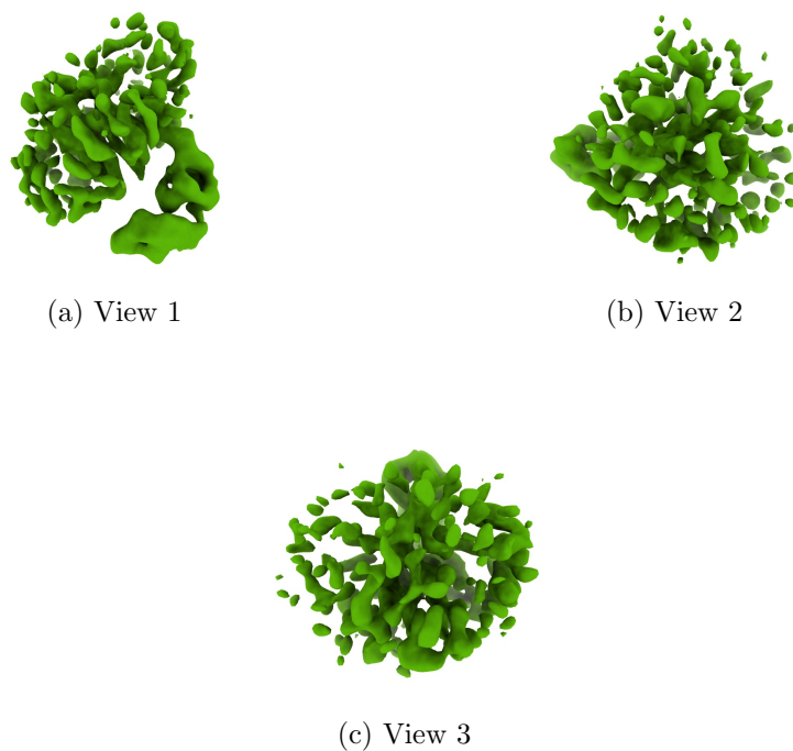
Figure 4: Isosurface at threshold=0.088000. Views generated by ChimeraX at a the following X, Y, Z angles: View 1 (0, -90, -90), View 2 (-90, 0, -90), View 3 (0, 0, 0).
