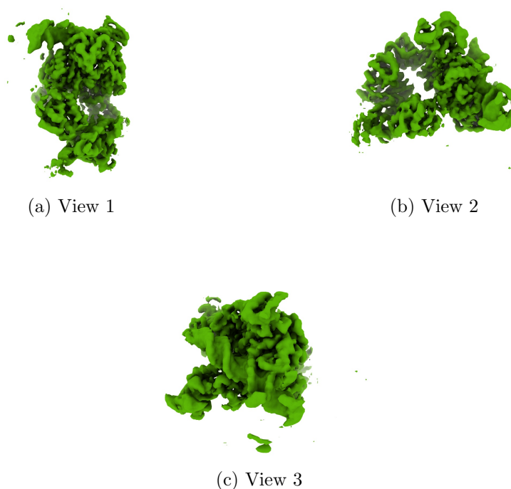
Figure 4: Isosurface at threshold=0.009000. Views generated by ChimeraX at a the following X, Y, Z angles: View 1 (0, -90, -90), View 2 (-90, 0, -90), View 3 (0, 0, 0).
