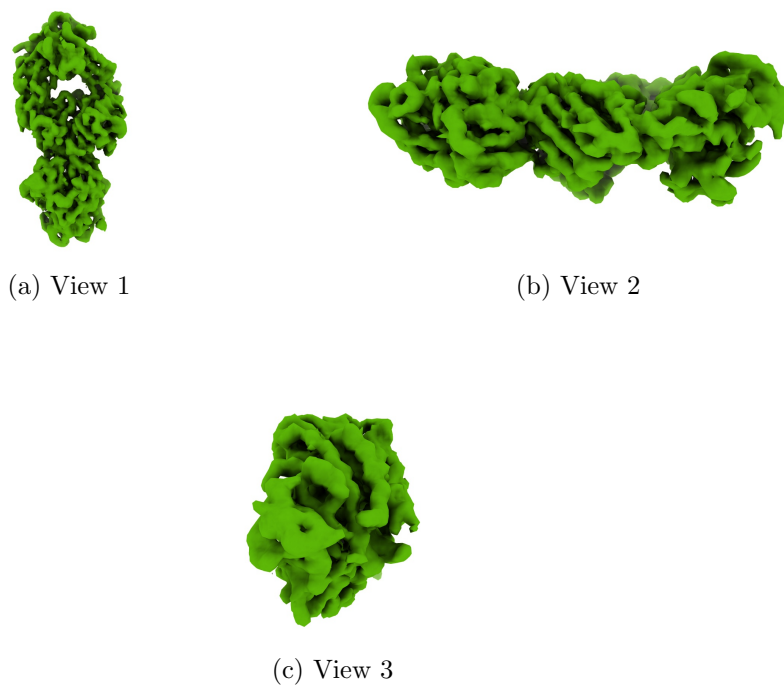
Figure 4: Isosurface at threshold=0.095000. Views generated by ChimeraX at a the following X, Y, Z angles: View 1 (0, -90, -90), View 2 (-90, 0, -90), View 3 (0, 0, 0).
