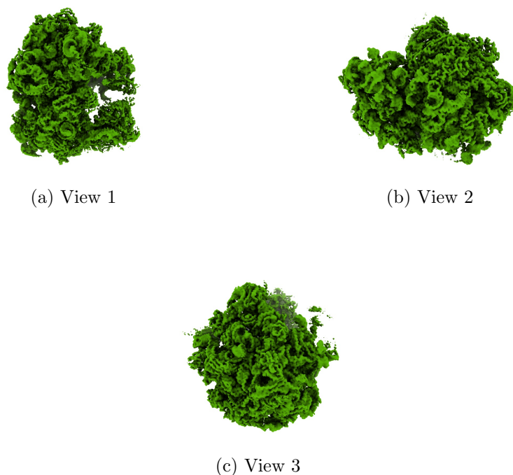
Figure 4: Isosurface at threshold=0.072000. Views generated by ChimeraX at a the following X, Y, Z angles: View 1 (0, -90, -90), View 2 (-90, 0, -90), View 3 (0, 0, 0).
