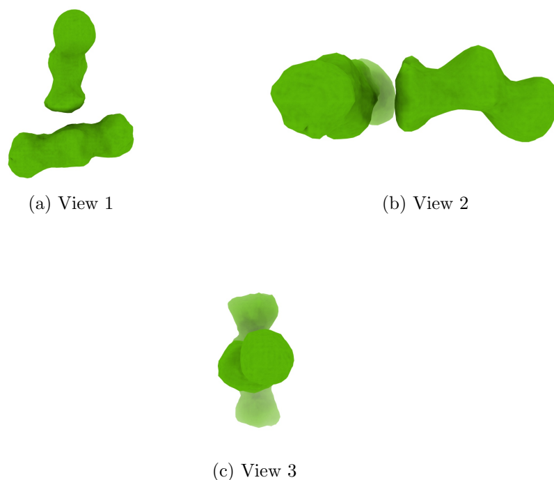
Figure 4: Isosurface at threshold=0.534000. Views generated by ChimeraX at a the following X, Y, Z angles: View 1 (0, -90, -90), View 2 (-90, 0, -90), View 3 (0, 0, 0).
