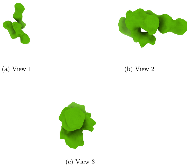
Figure 4: Isosurface at threshold=0.796000. Views generated by ChimeraX at a the following X, Y, Z angles: View 1 (0, -90, -90), View 2 (-90, 0, -90), View 3 (0, 0, 0).
