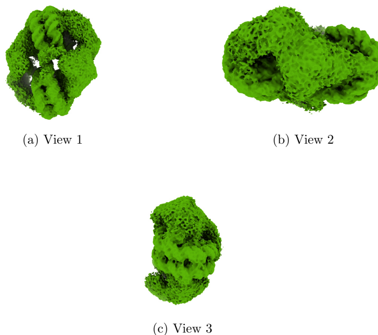
Figure 4: Isosurface at threshold=0.023800. Views generated by ChimeraX at a the following X, Y, Z angles: View 1 (0, -90, -90), View 2 (-90, 0, -90), View 3 (0, 0, 0).
