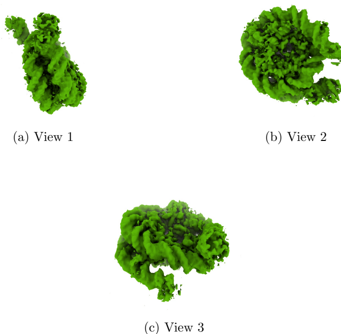
Figure 4: Isosurface at threshold=0.028800. Views generated by ChimeraX at a the following X, Y, Z angles: View 1 (0, -90, -90), View 2 (-90, 0, -90), View 3 (0, 0, 0).
