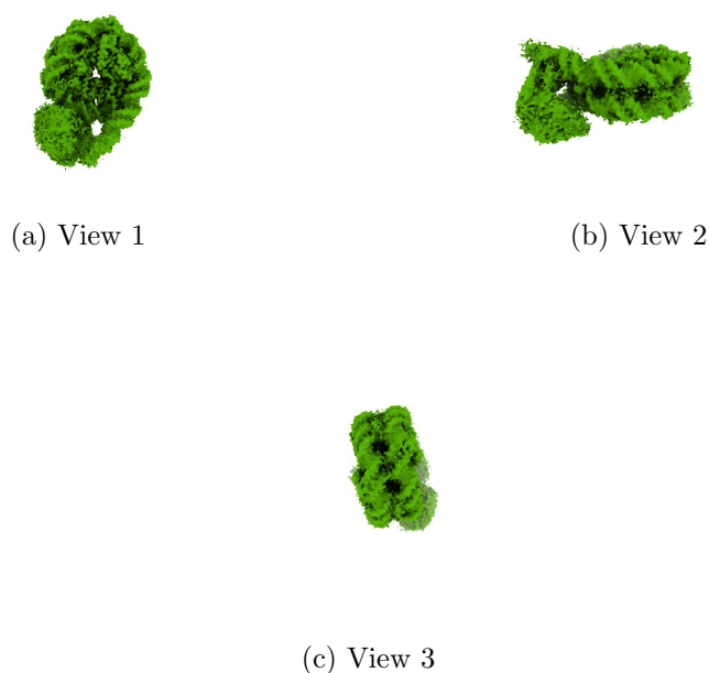
Figure 4: Isosurface at threshold=0.002940. Views generated by ChimeraX at a the following X, Y, Z angles: View 1 (0, -90, -90), View 2 (-90, 0, -90), View 3 (0, 0, 0).
